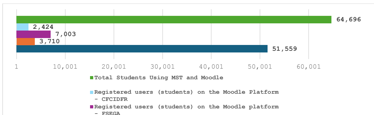
Figure 11. LMS users.
